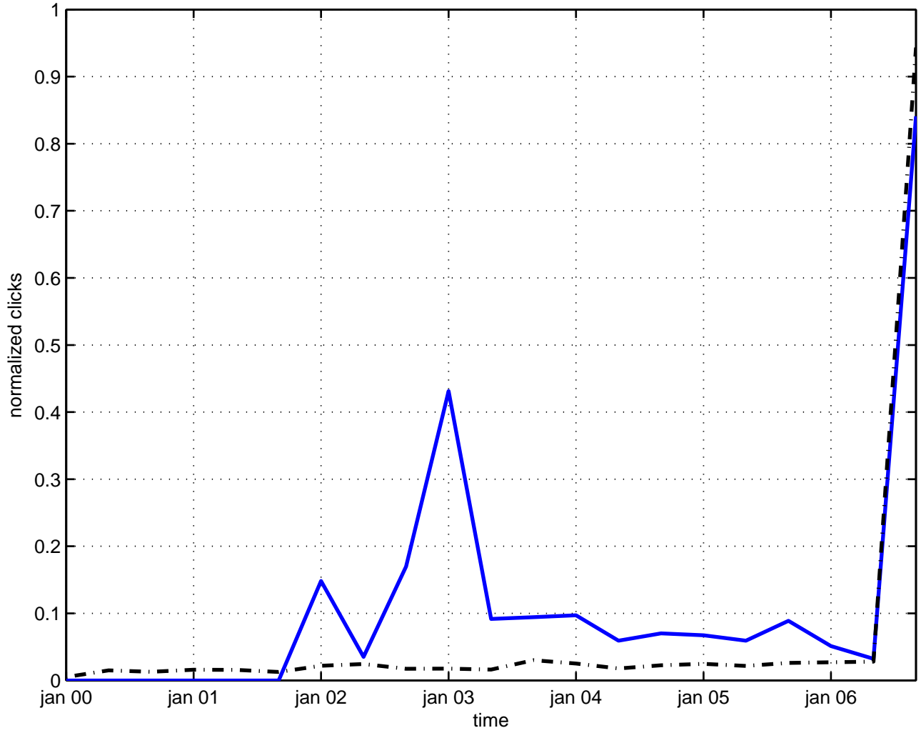
parasupersymmetry
