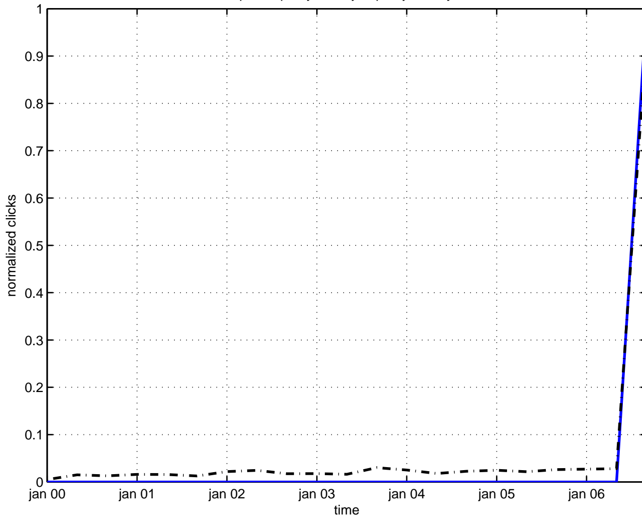
parasupersymmetry supersymmetry
