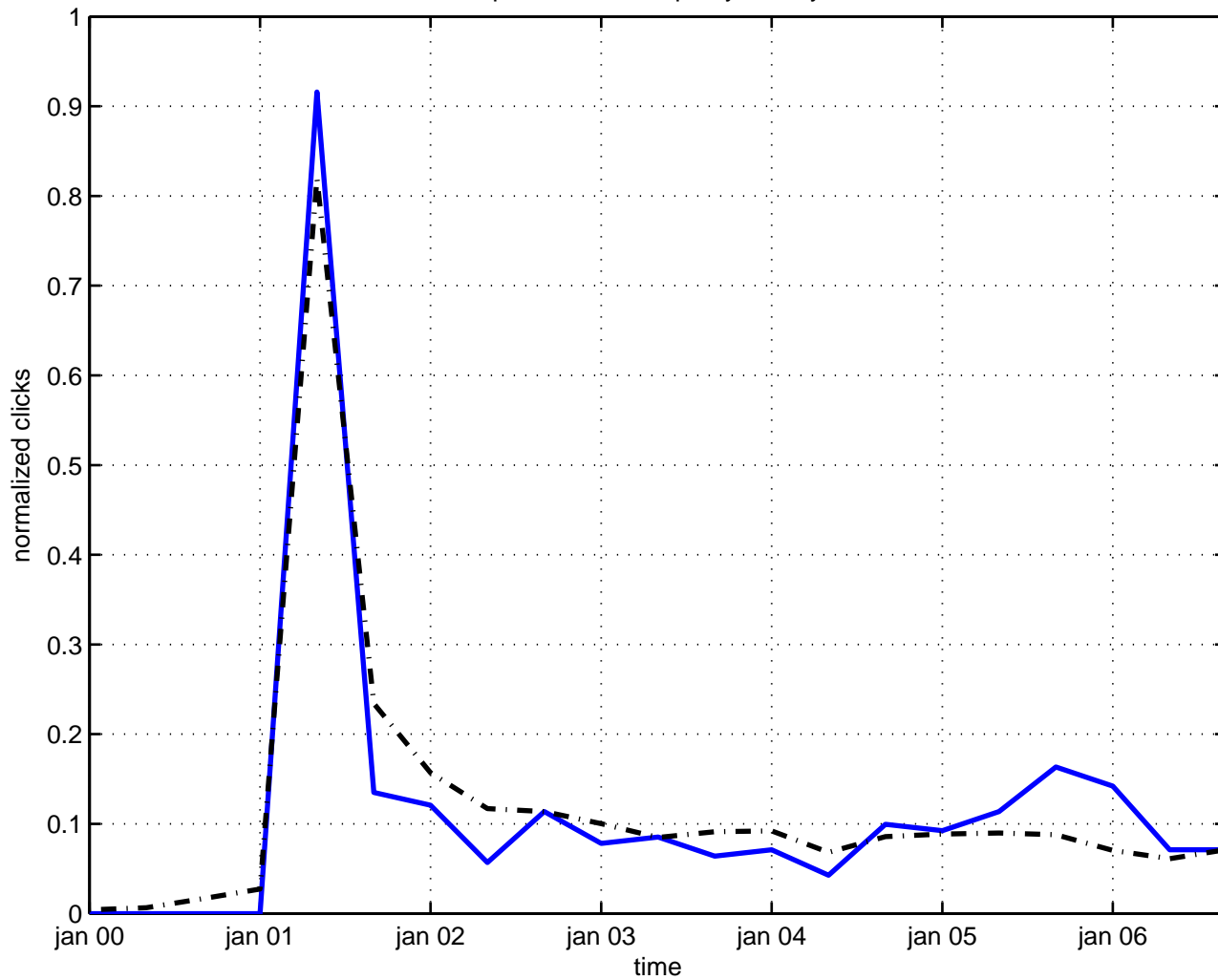
parastatistics supersymmetry
