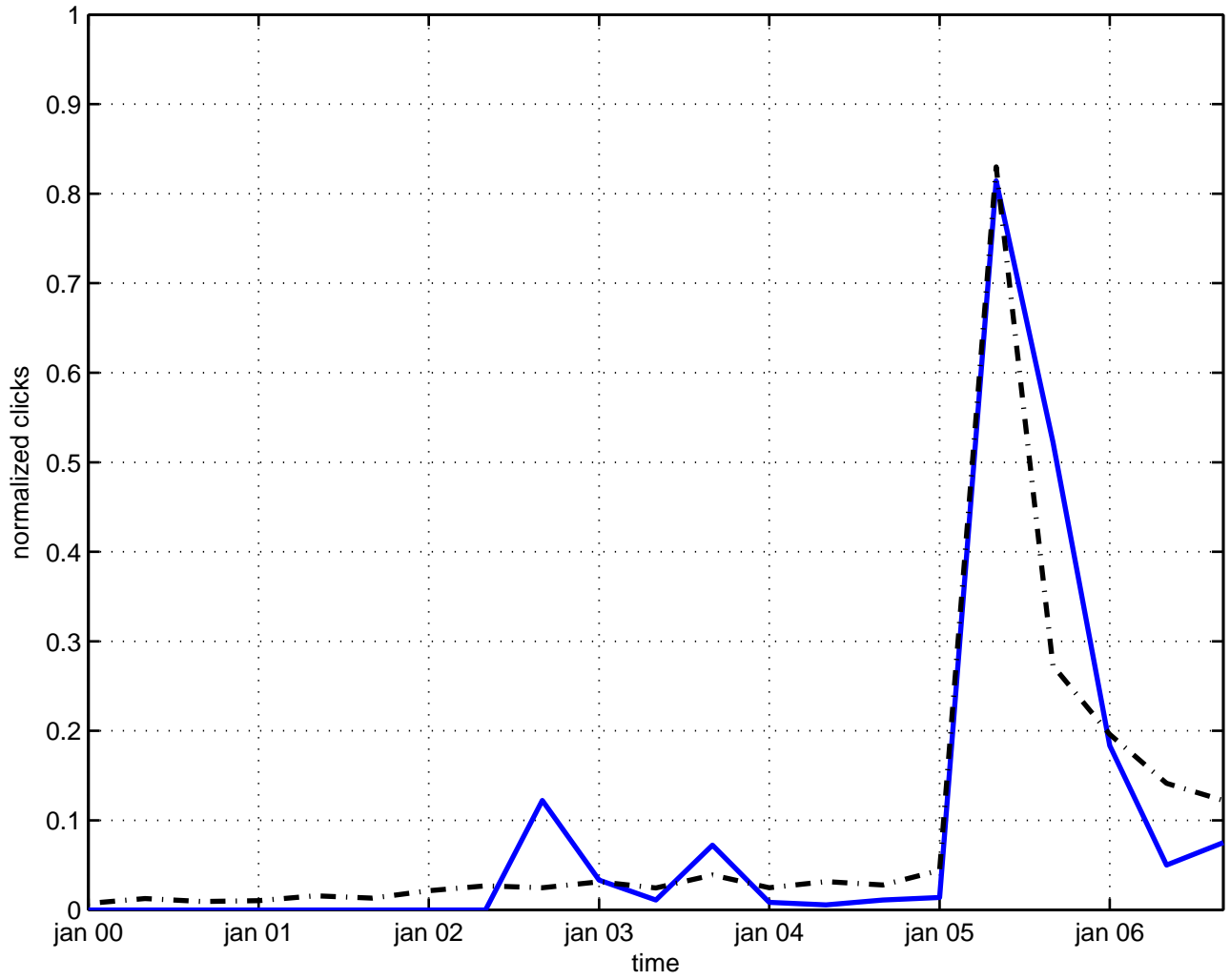
parastatistics boson
