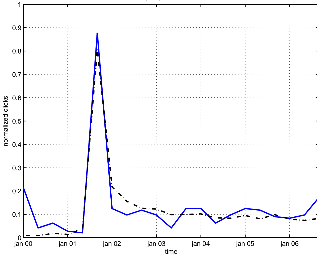
pair production w
