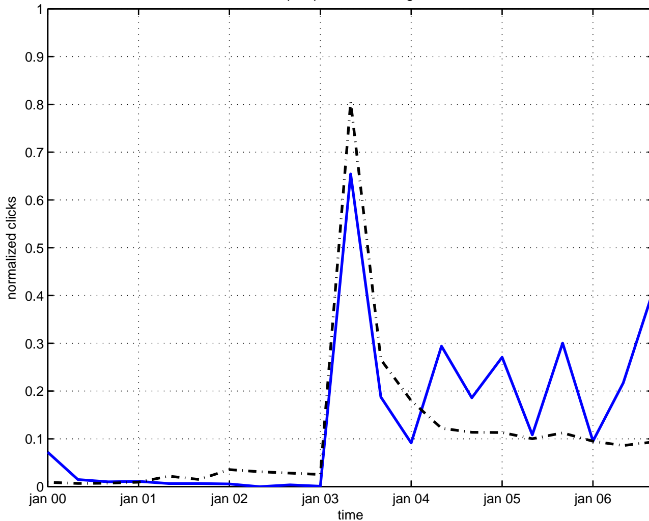
pair production string
