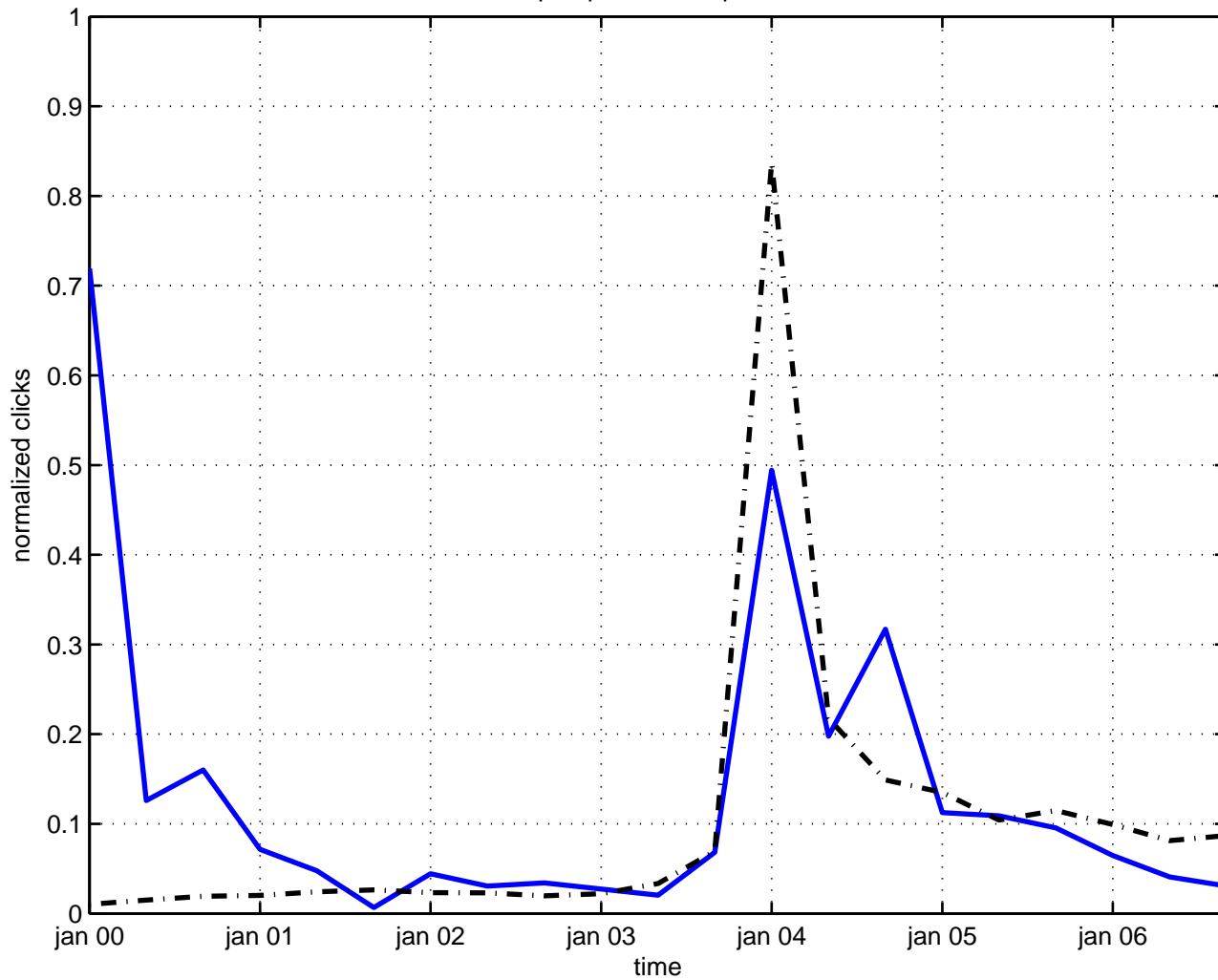
pair production quark
