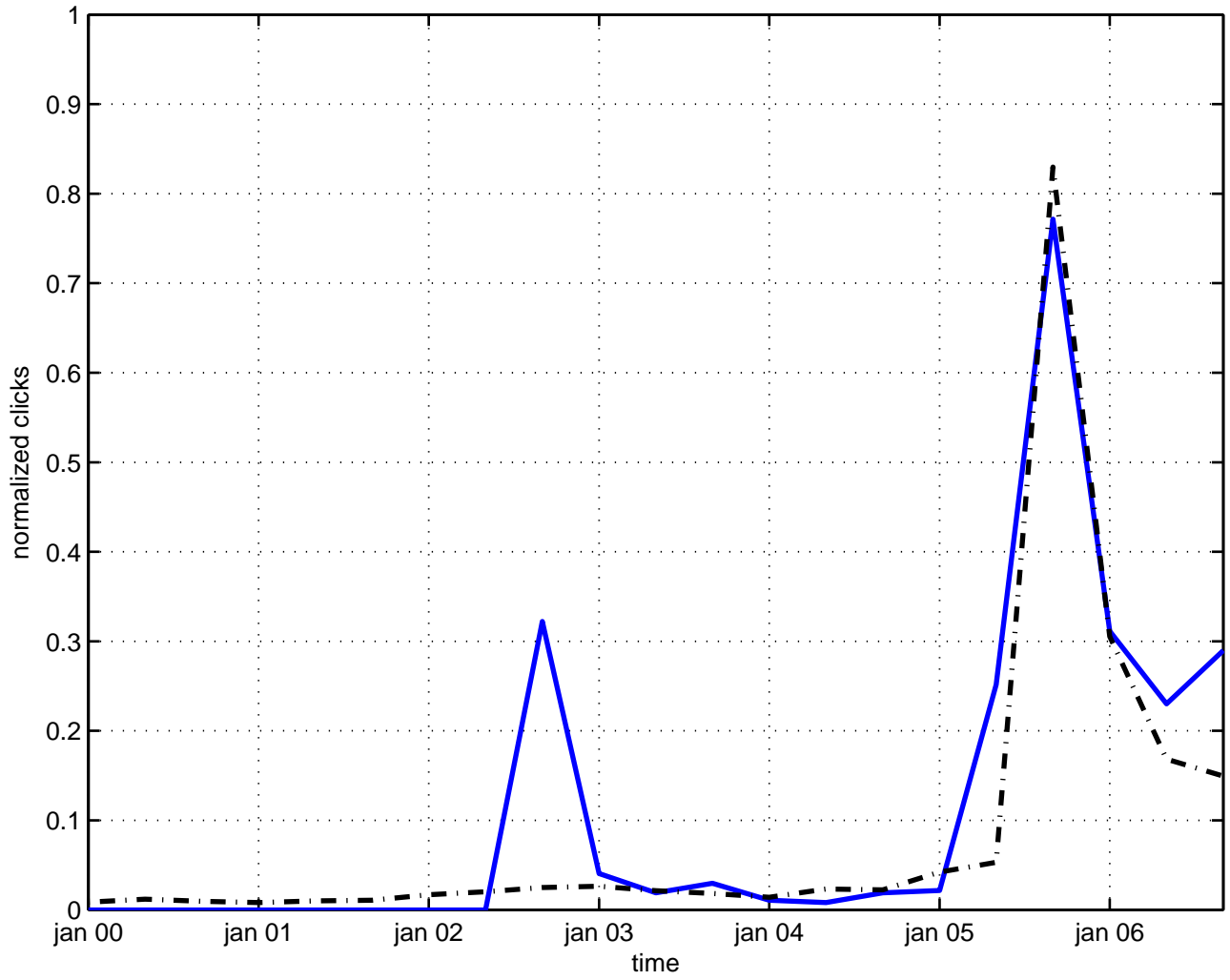
pair production photon
