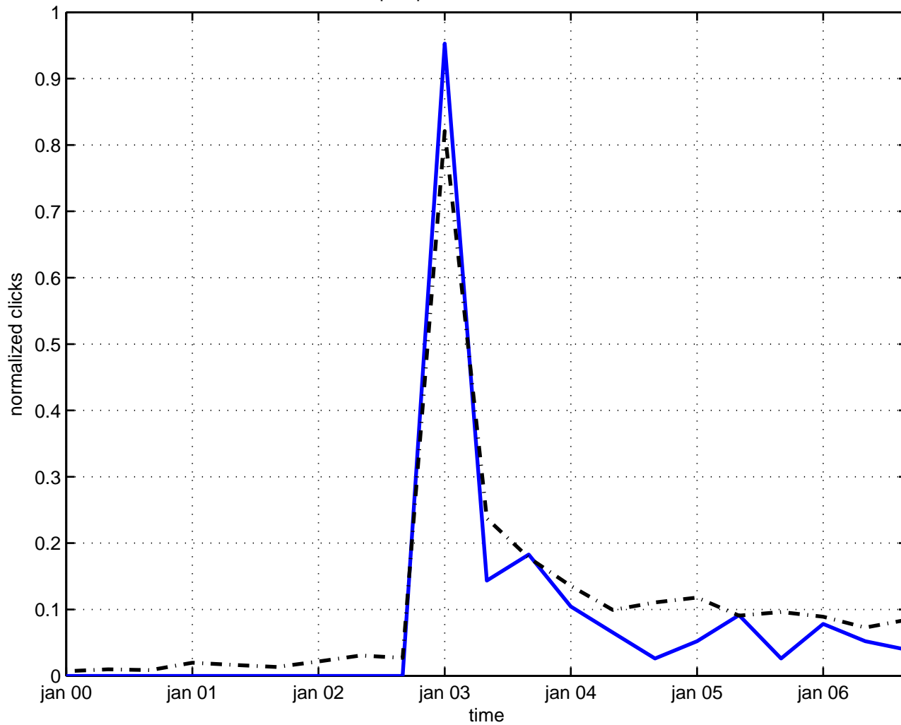
pair production neutrino/e
