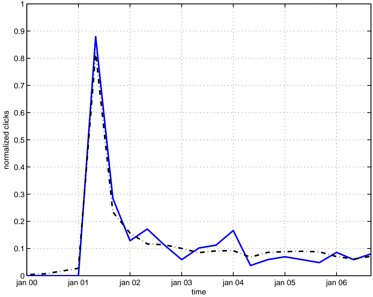
pair production magnetic monopole
