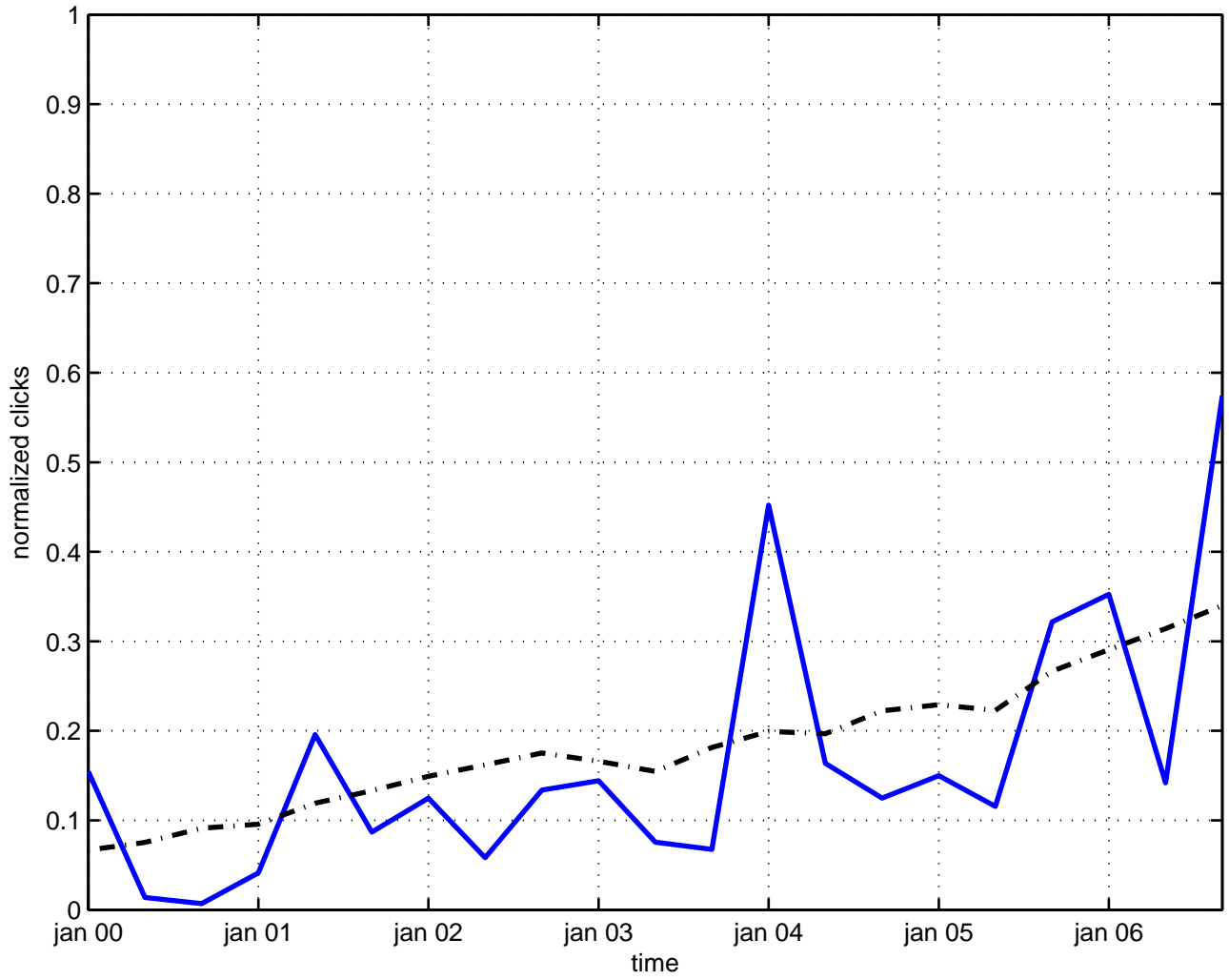
pair production electron
