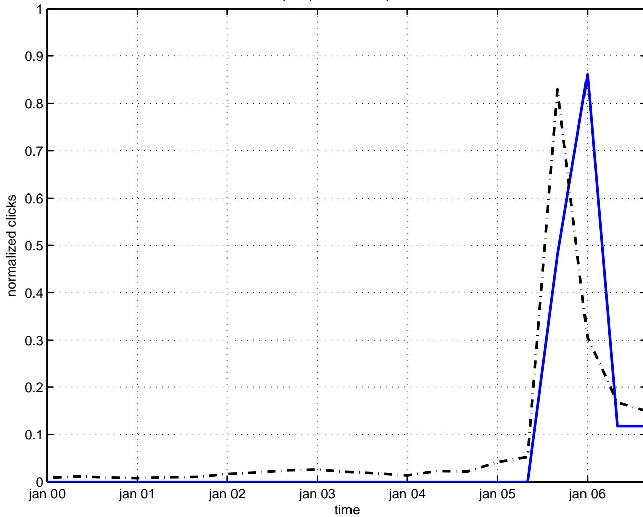
pair production dipole
