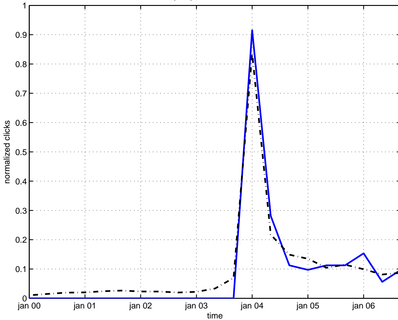
pair production bubble
