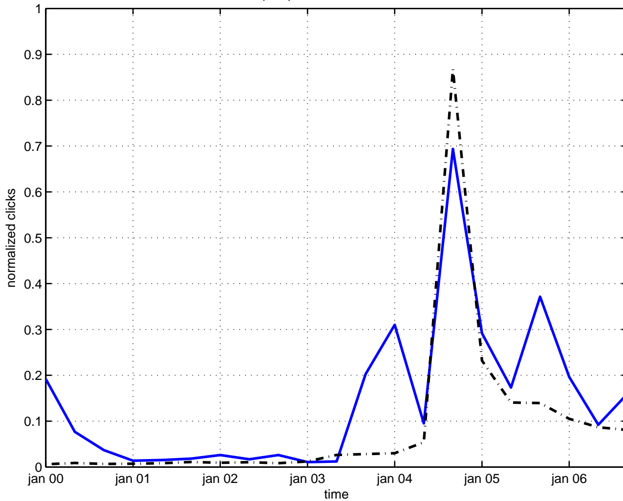
pair production black hole
