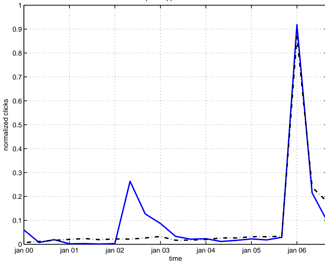
pade approximation
