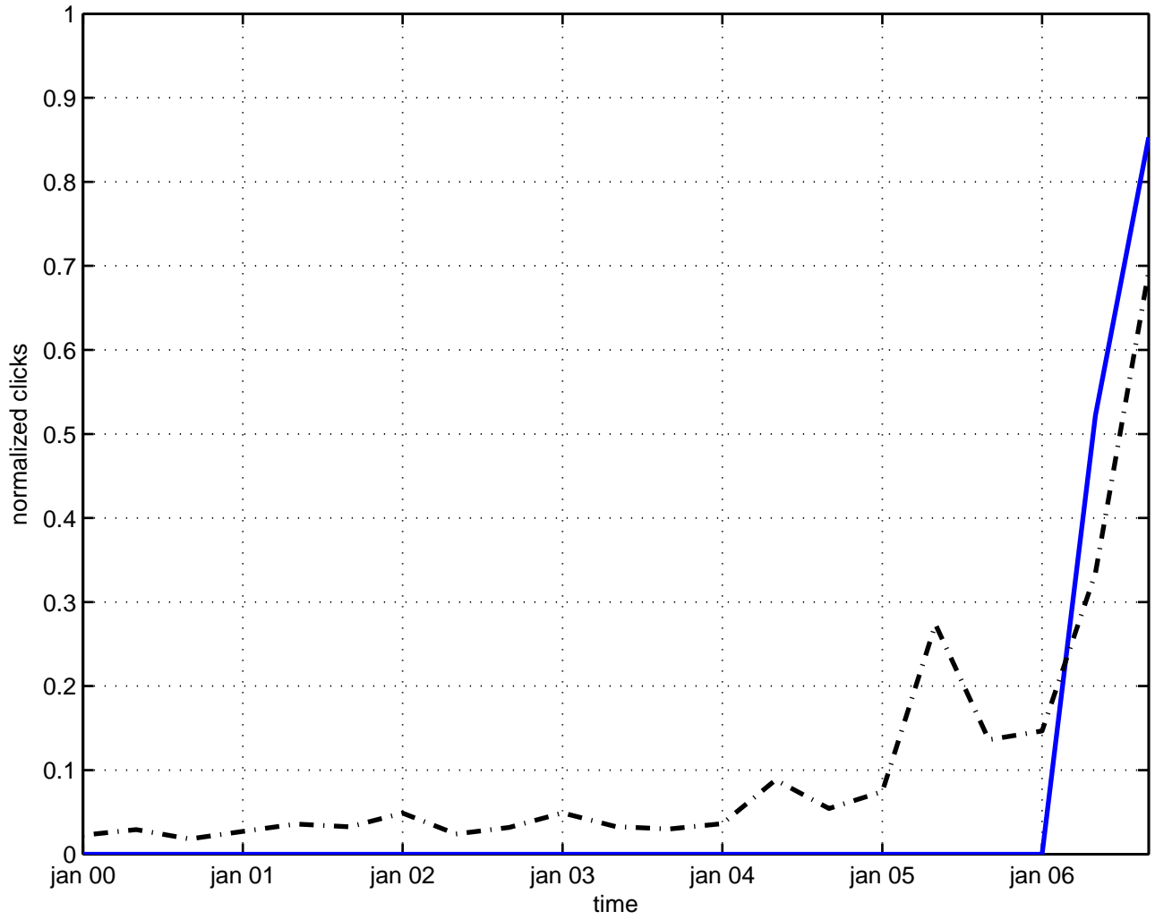
overlap fermion
