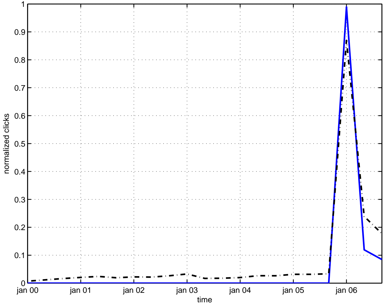
osp(n|m) gauge field theory
