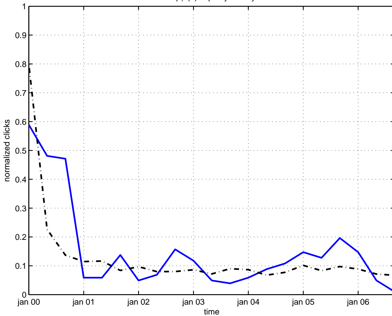
osp(4|2) supersymmetry
