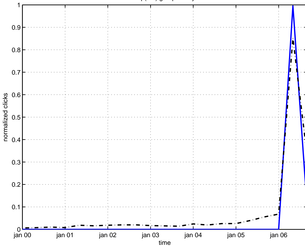
osp(4/4) group theory
