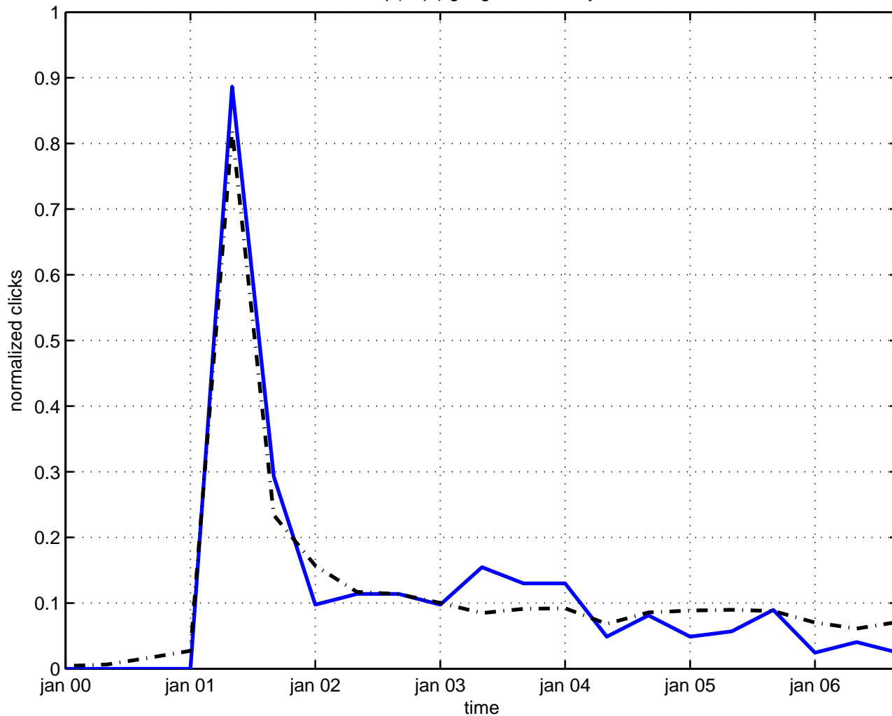
osp(32|1) gauge field theory
