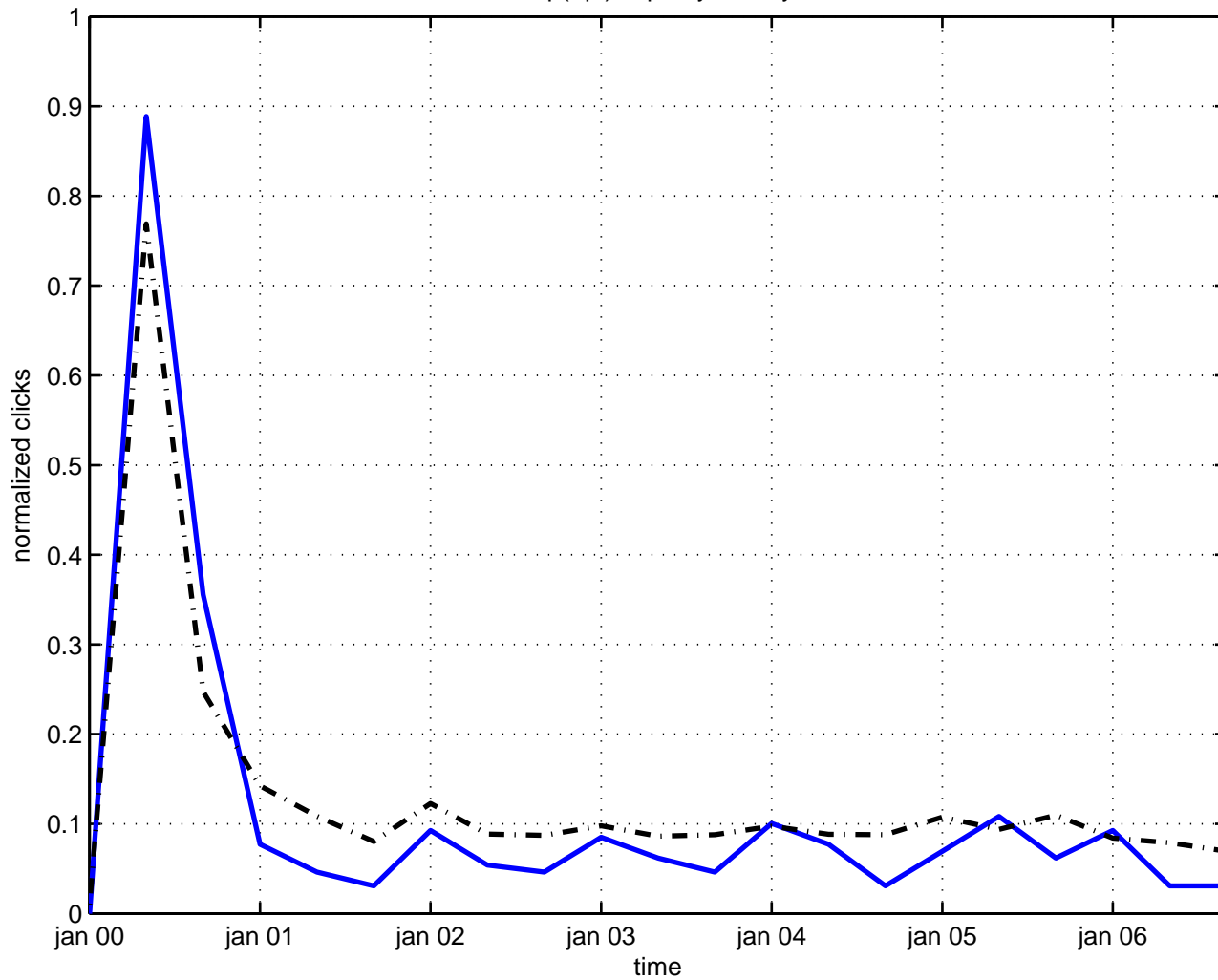
osp(2|2) supersymmetry
