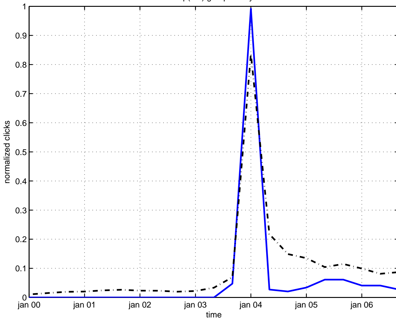
osp(2/2) group theory
