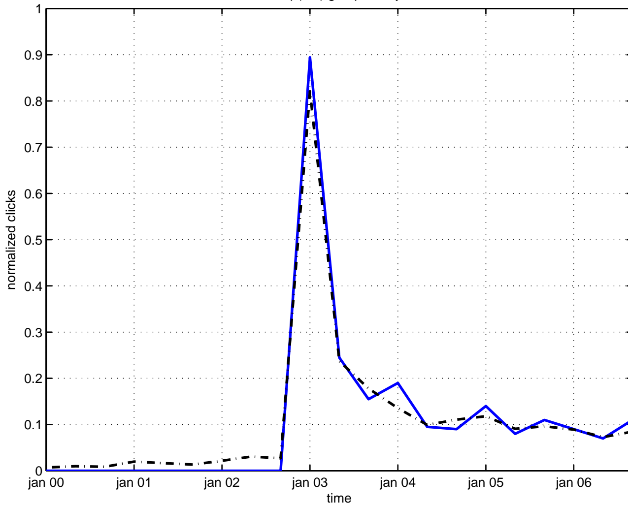
osp(1/2) group theory
