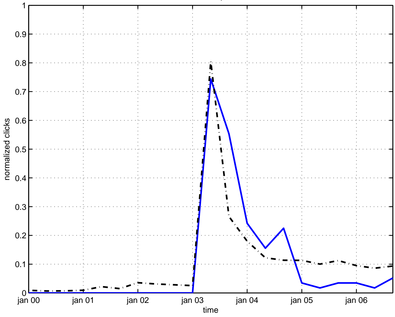
oscillator quark
