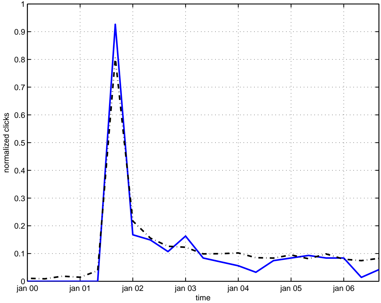
oscillator quantum mechanics
