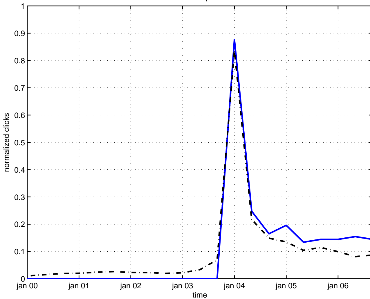
oscillation spectrum
