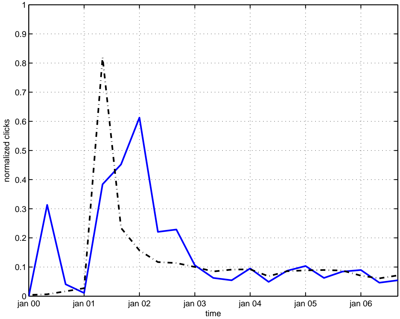
oscillation space-time
