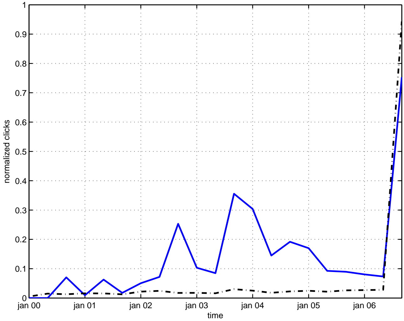
oscillation neutrino
