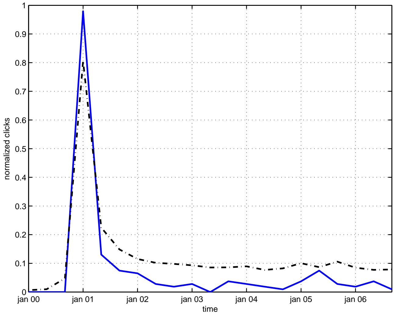
oscillation model
