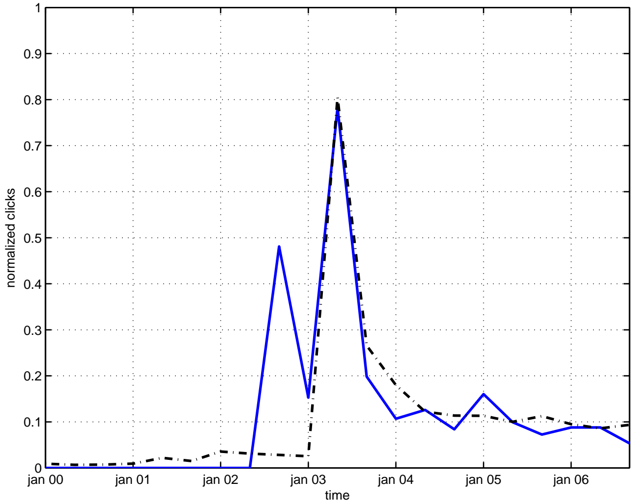
oscillation graviton
