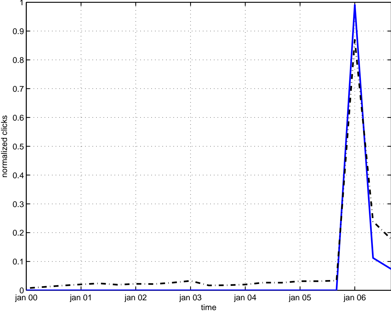
oscillation dark energy
