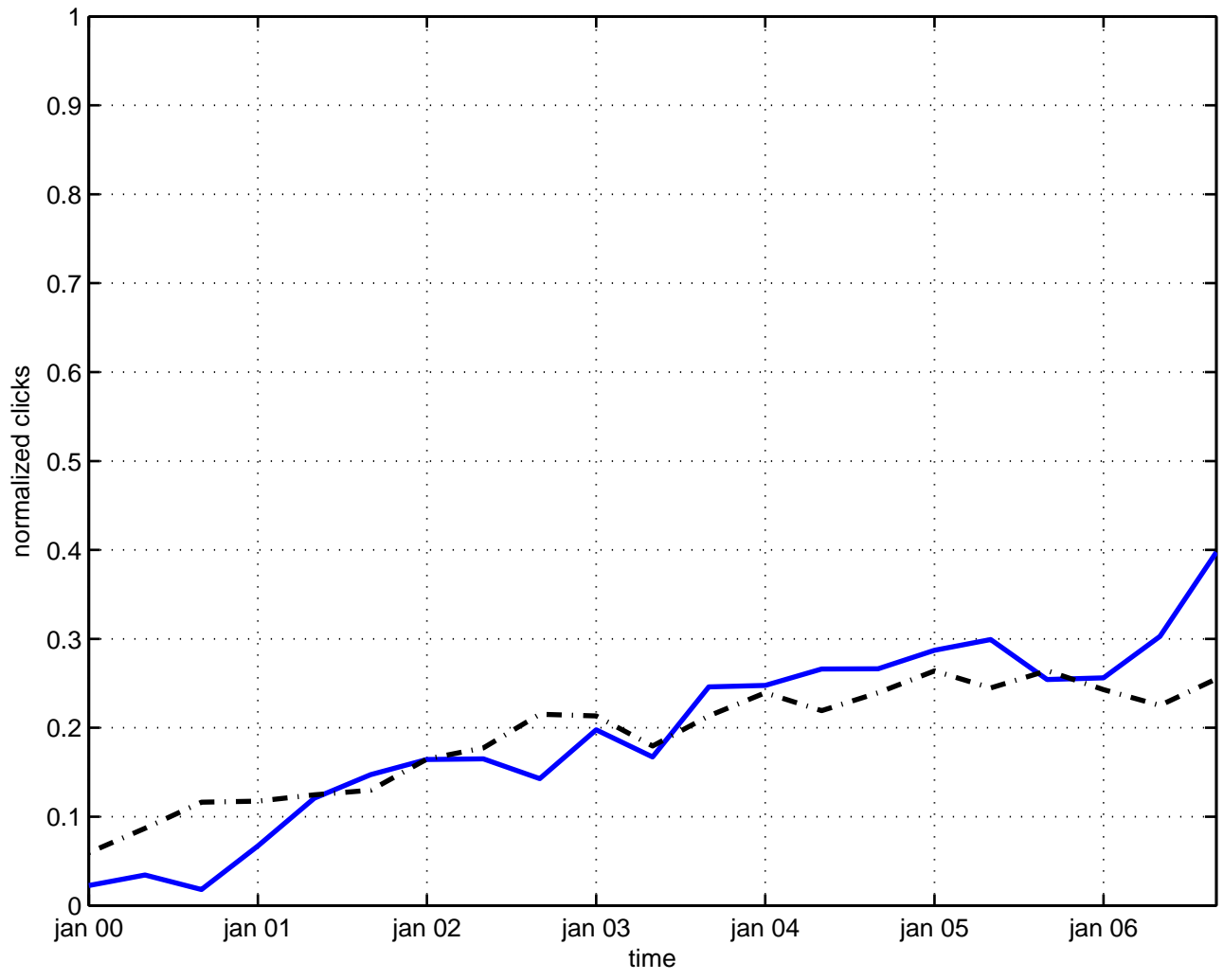
orientifold
