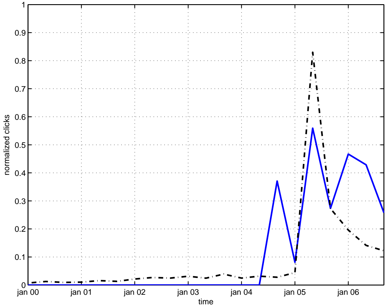
orientifold compactification
