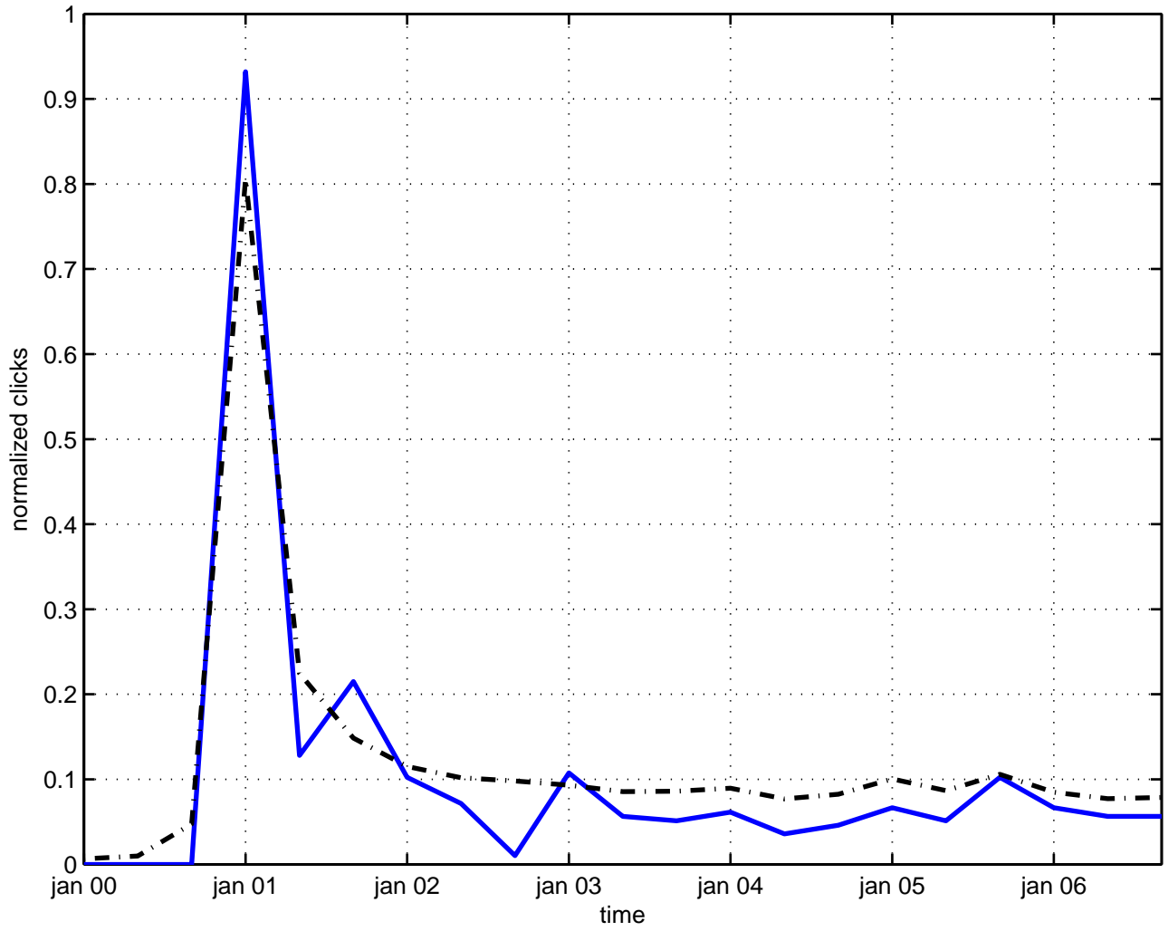
orbifold string
