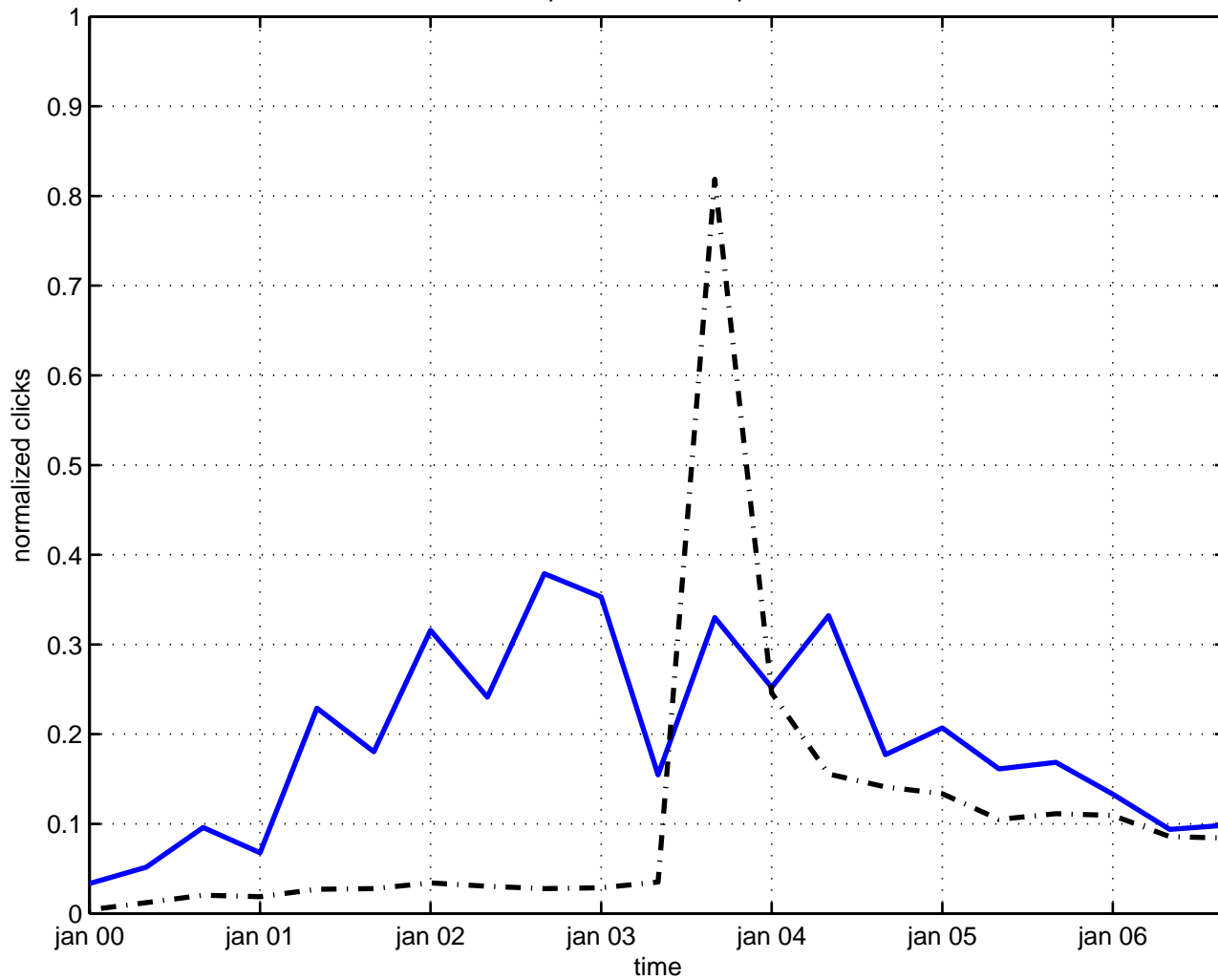
orbifold spontaneous compactification
