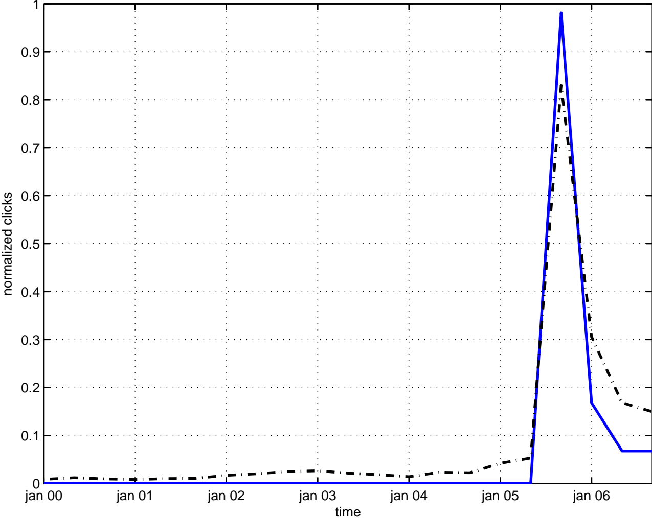
orbifold space-time
