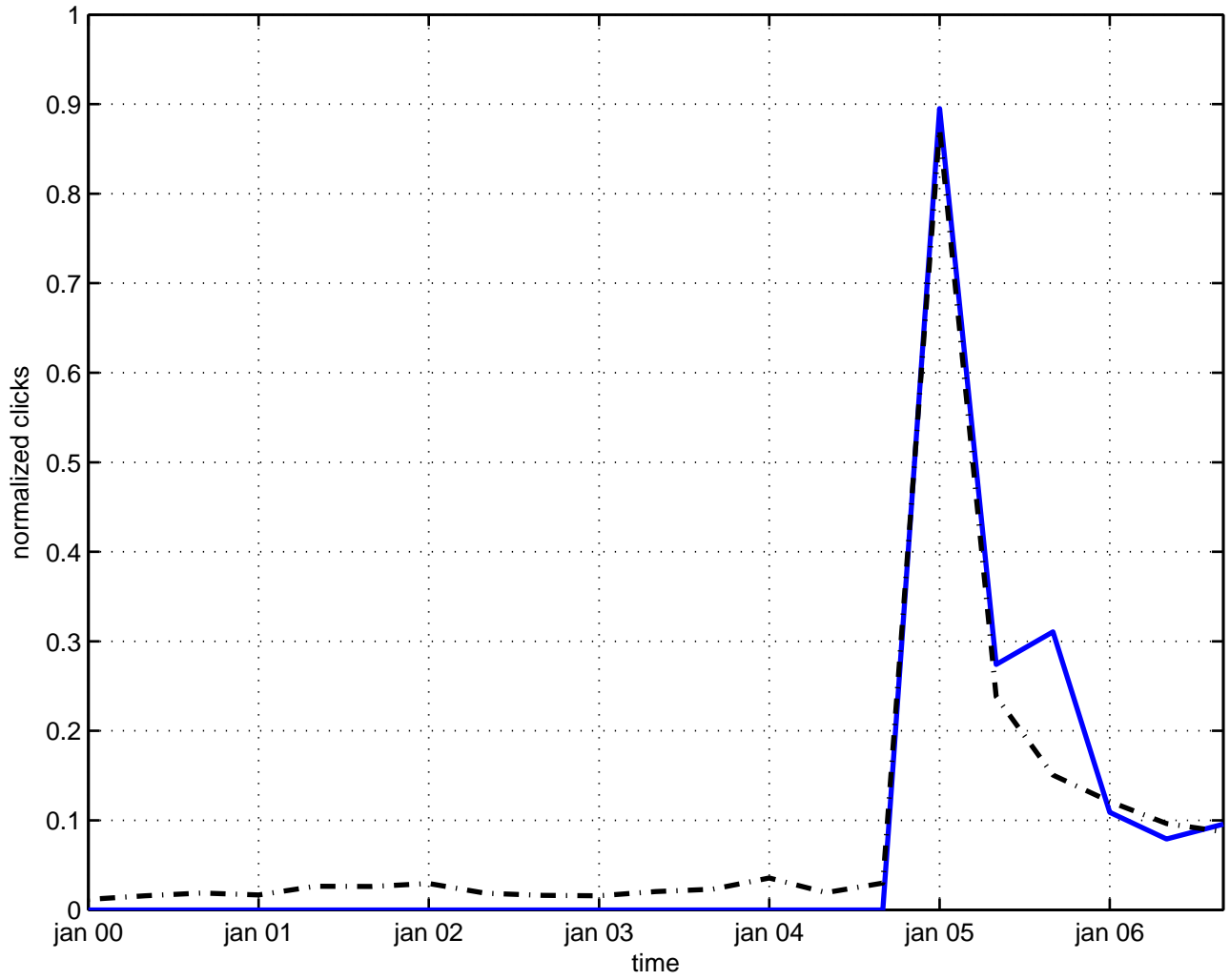
orbifold conifold
