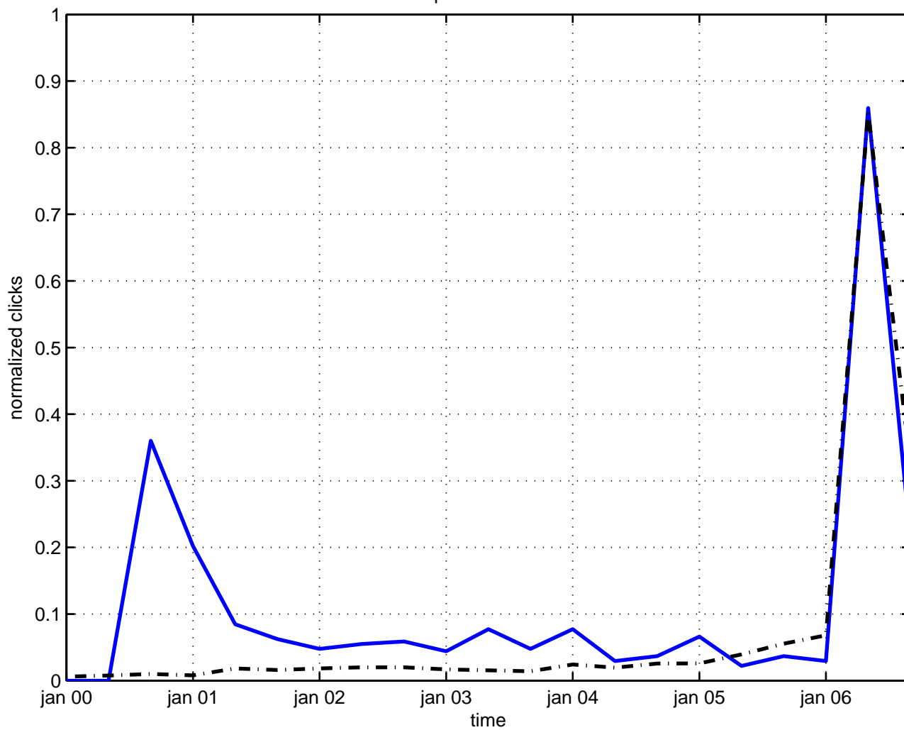
optical theorem
