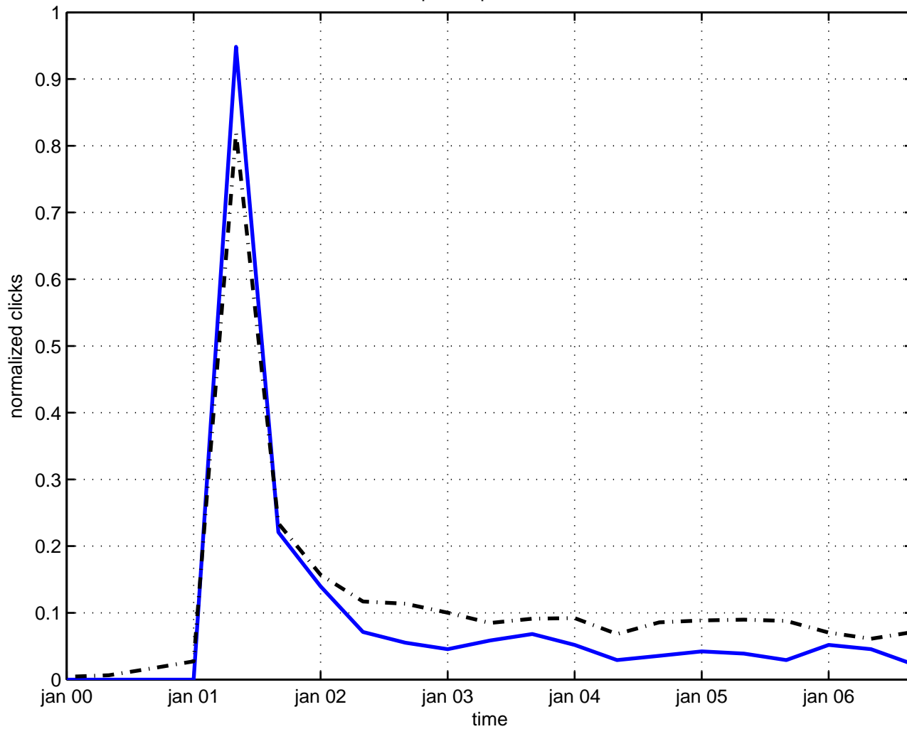
optical space-time
