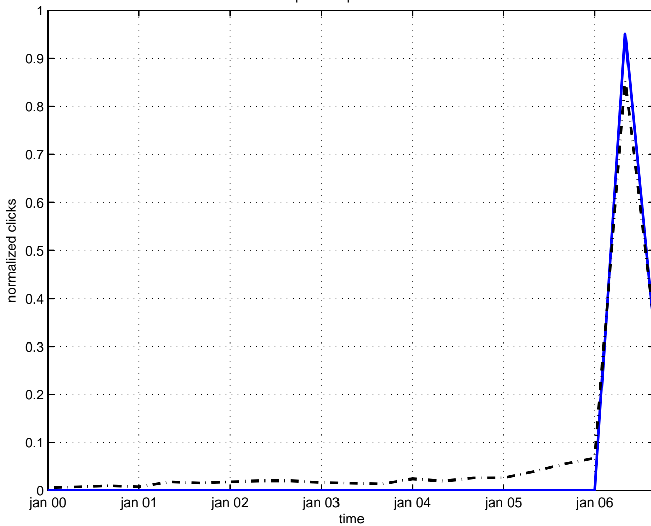
operator quantization
