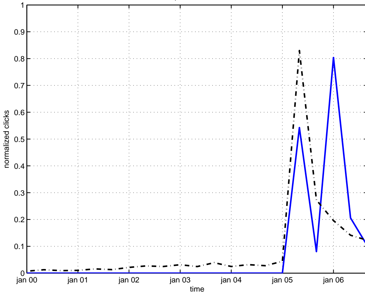
operator meson
