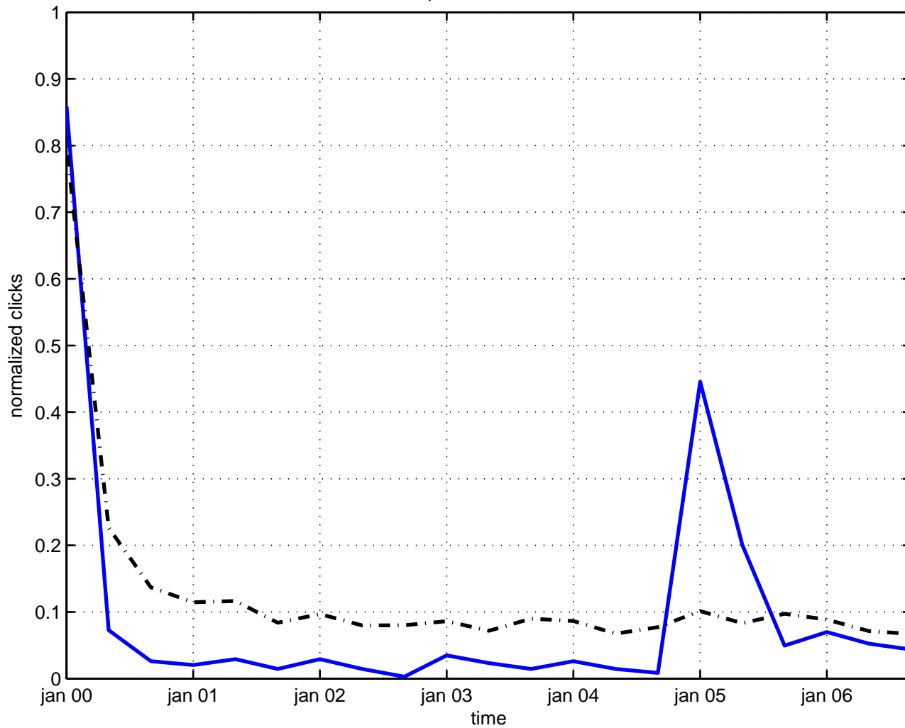
operator electron
