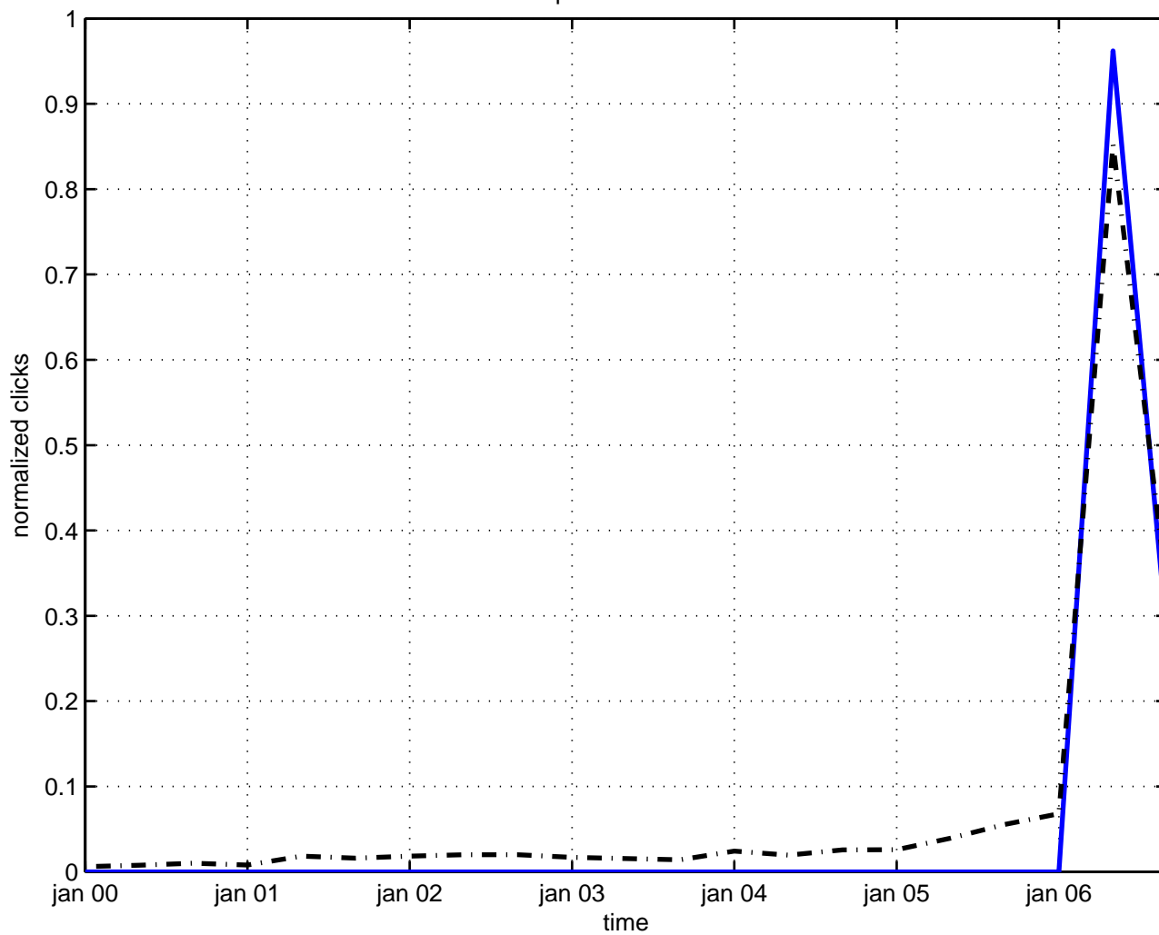
operator dilaton
