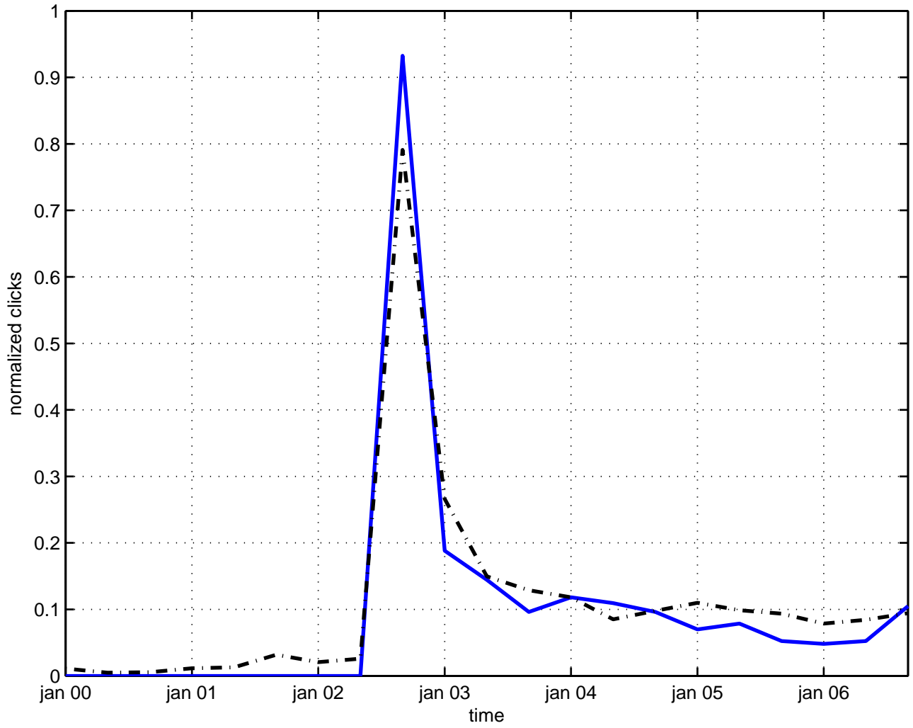
operator angular momentum
