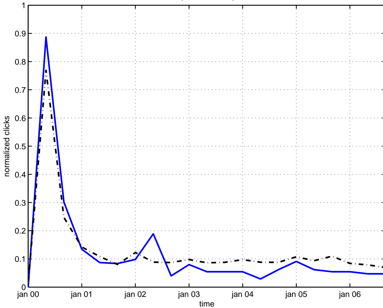
open wilson loop
