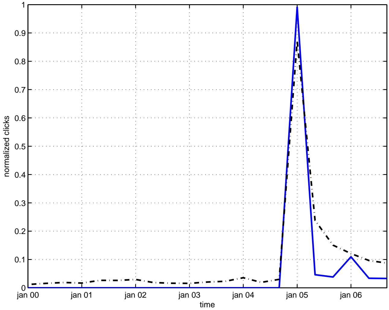
one-pion exchange
