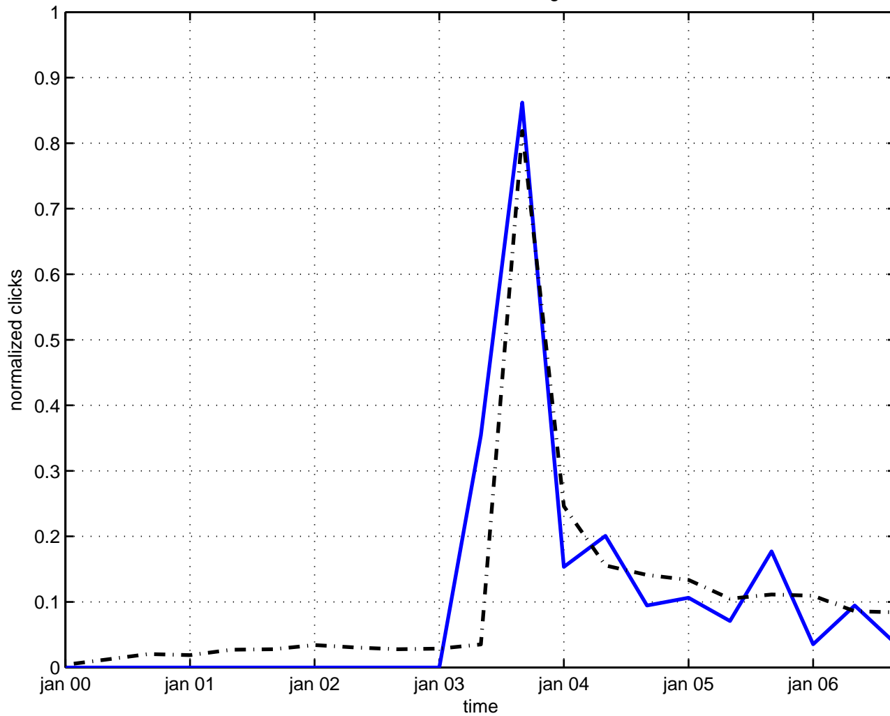
one-boson exchange
