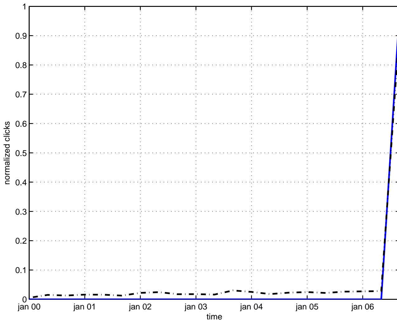
on-shell renormalization
