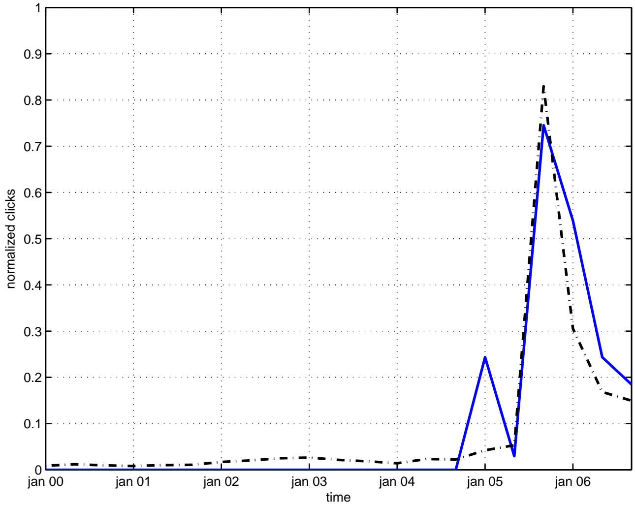
off-shell supersymmetry
