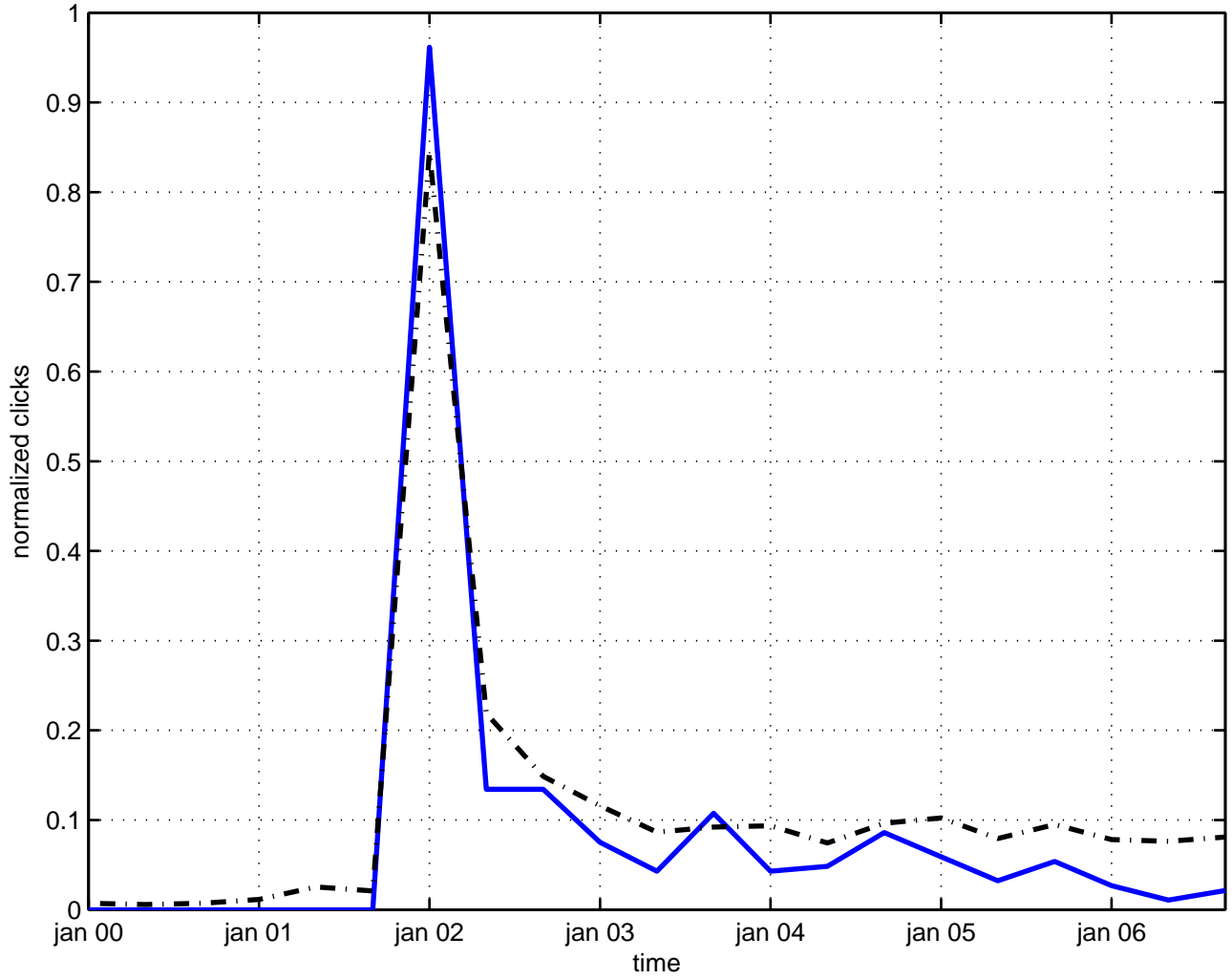
off-shell correlation function
